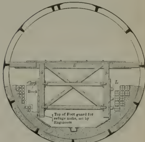
SECTION SHOWING FORMS FOR BENCH FIG. 2
